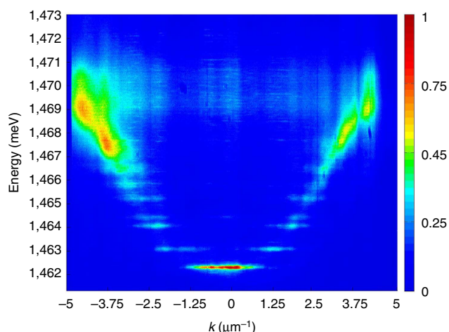
Figure 1 | Energy modes separation. Dispersion curve for the 6 \mu\text{m} circular pillar used in the experiment (–5 meV cavity detuning), obtained with a non-resonant pumping at 1,550 meV. The lower polariton branch with several spatial modes and the weakly excited upper branch are visible. The modes are energetically separated and squeezing is protected against multimode nonlinear coupling.
